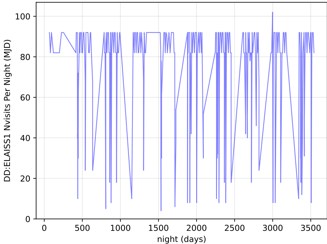
too_elab_r32_d3_gz_v3.4_10yrs all bands: DD:ELAISS1 Nvisits Per Night
