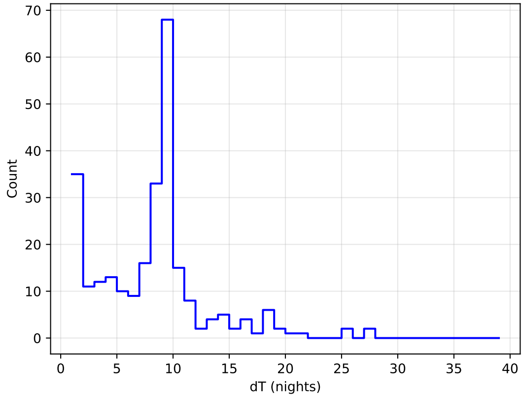
too_elab_r32_d3_gz_v3.4_10yrs all bands: DD:ELAISS1 Delta Nights Histogram
