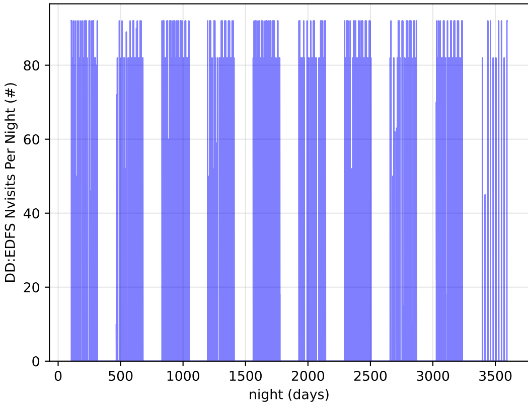
too_elab_r32_d3_gz_v3.4_10yrs all bands: DD:EDFS Nvisits Per Night
