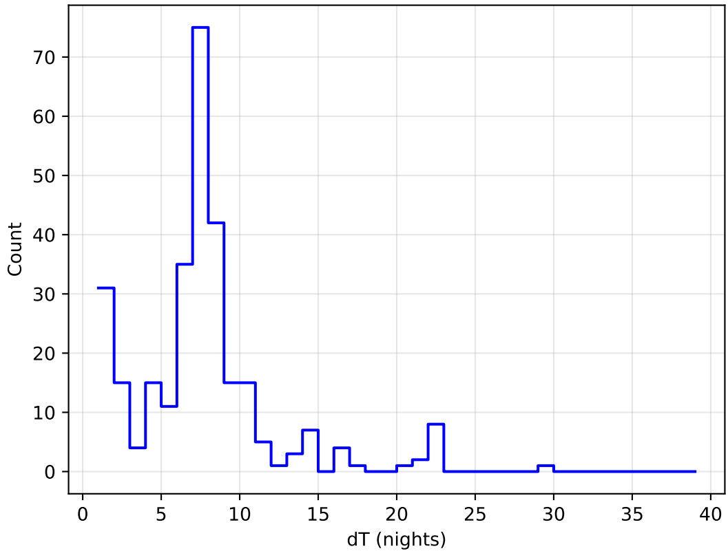
too_elab_r32_d3_gz_v3.4_10yrs all bands: DD:EDFS Delta Nights Histogram
