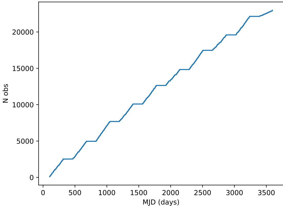
too_elab_r32_d3_gz_v3.4_10yrs all bands: DD:EDFS Cumulative NVisits
