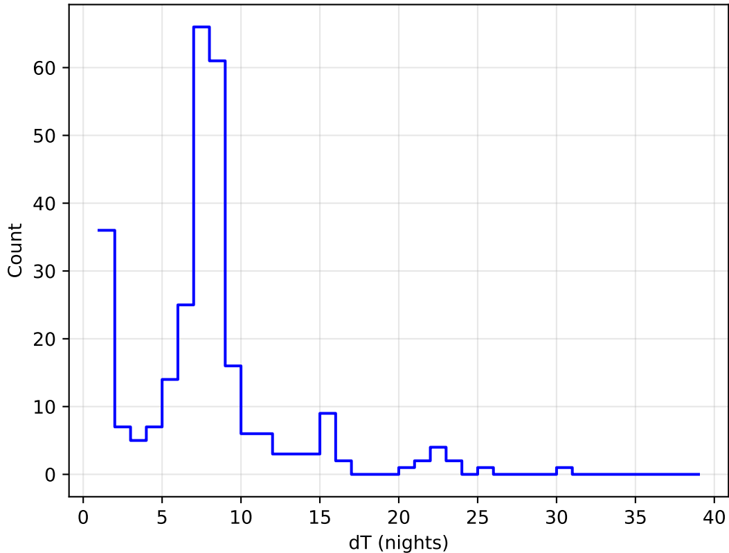
too_elab_r32_d3_gz_v3.4_10yrs all bands: DD:ECDFS Delta Nights Histogram
