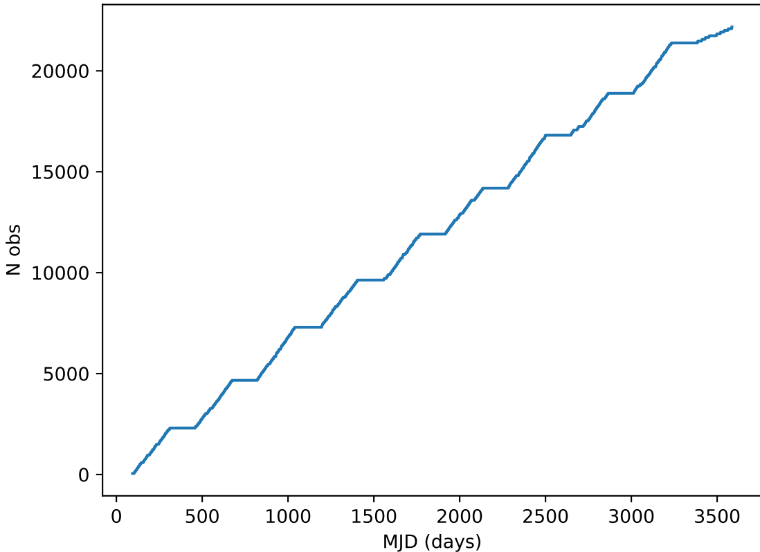
too_elab_r32_d3_gz_v3.4_10yrs all bands: DD:ECDFS Cumulative NVisits
