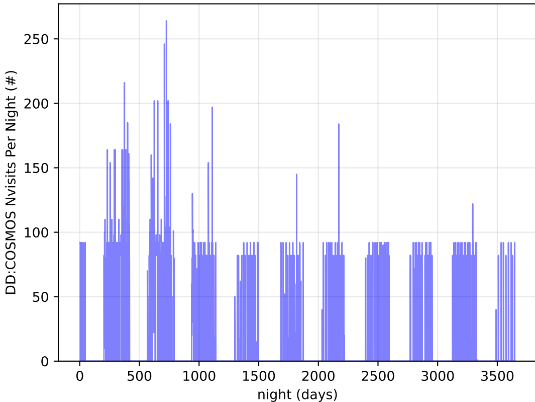
too_elab_r32_d3_gz_v3.4_10yrs all bands: DD: COSMOS Nvisits Per Night
