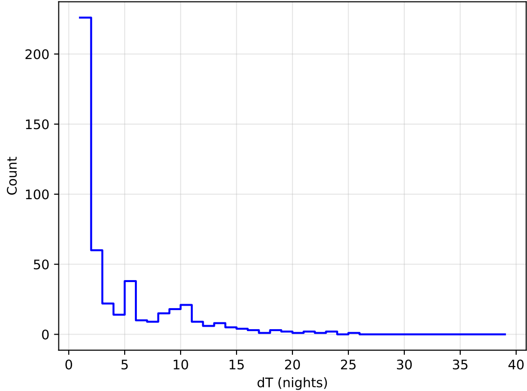
too_elab_r32_d3_gz_v3.4_10yrs all bands: DD: COSMOS Delta Nights Histogram
