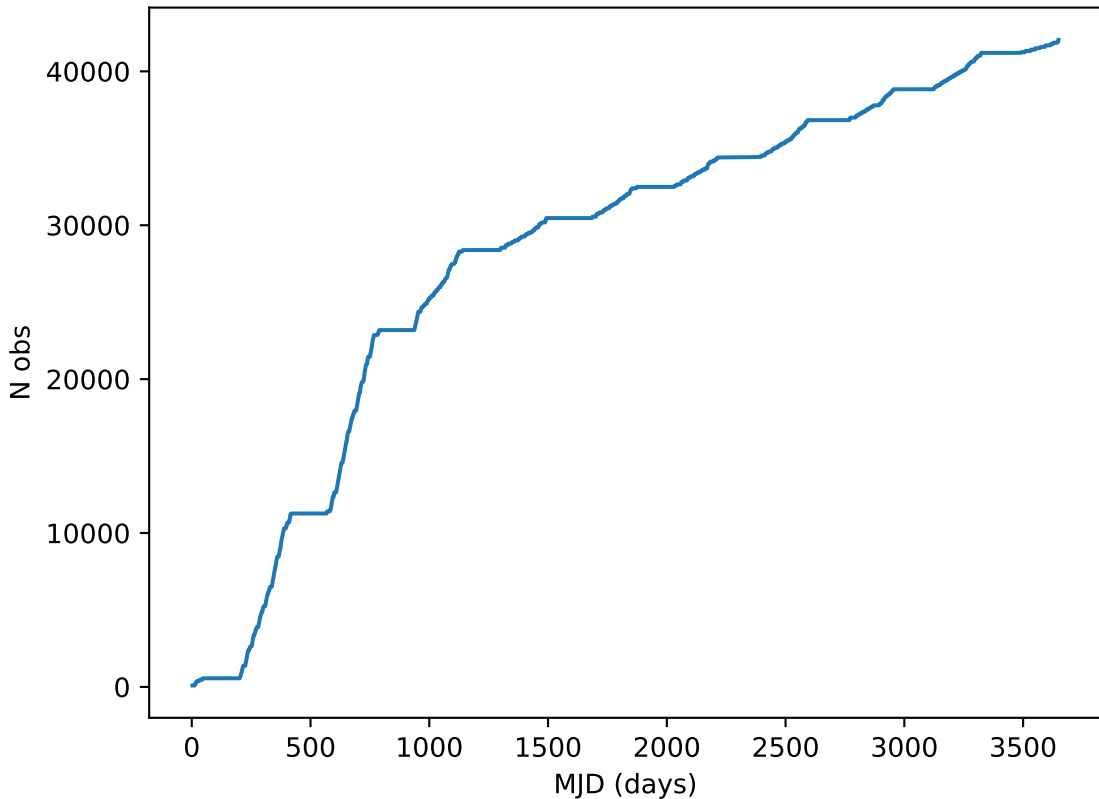
too_elab_r32_d3_gz_v3.4_10yrs all bands: DD: COSMOS Cumulative NVisits
