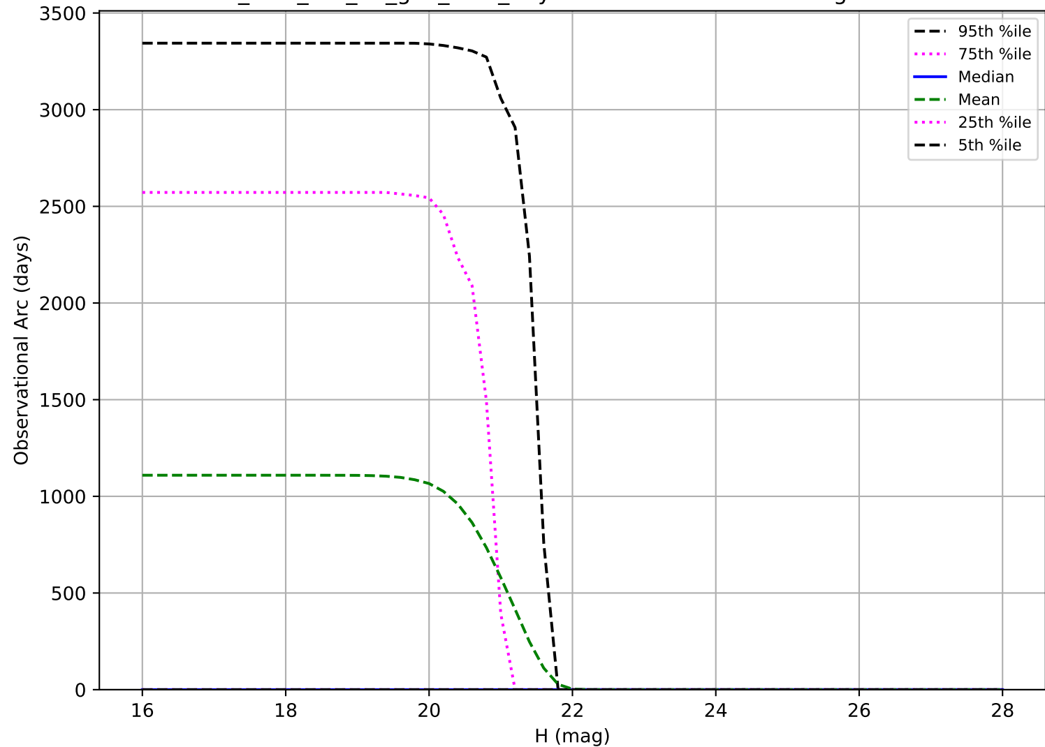
too_elab_r32_d3_griz_v3.4_10yrs: Observational Arc Length Vatira
