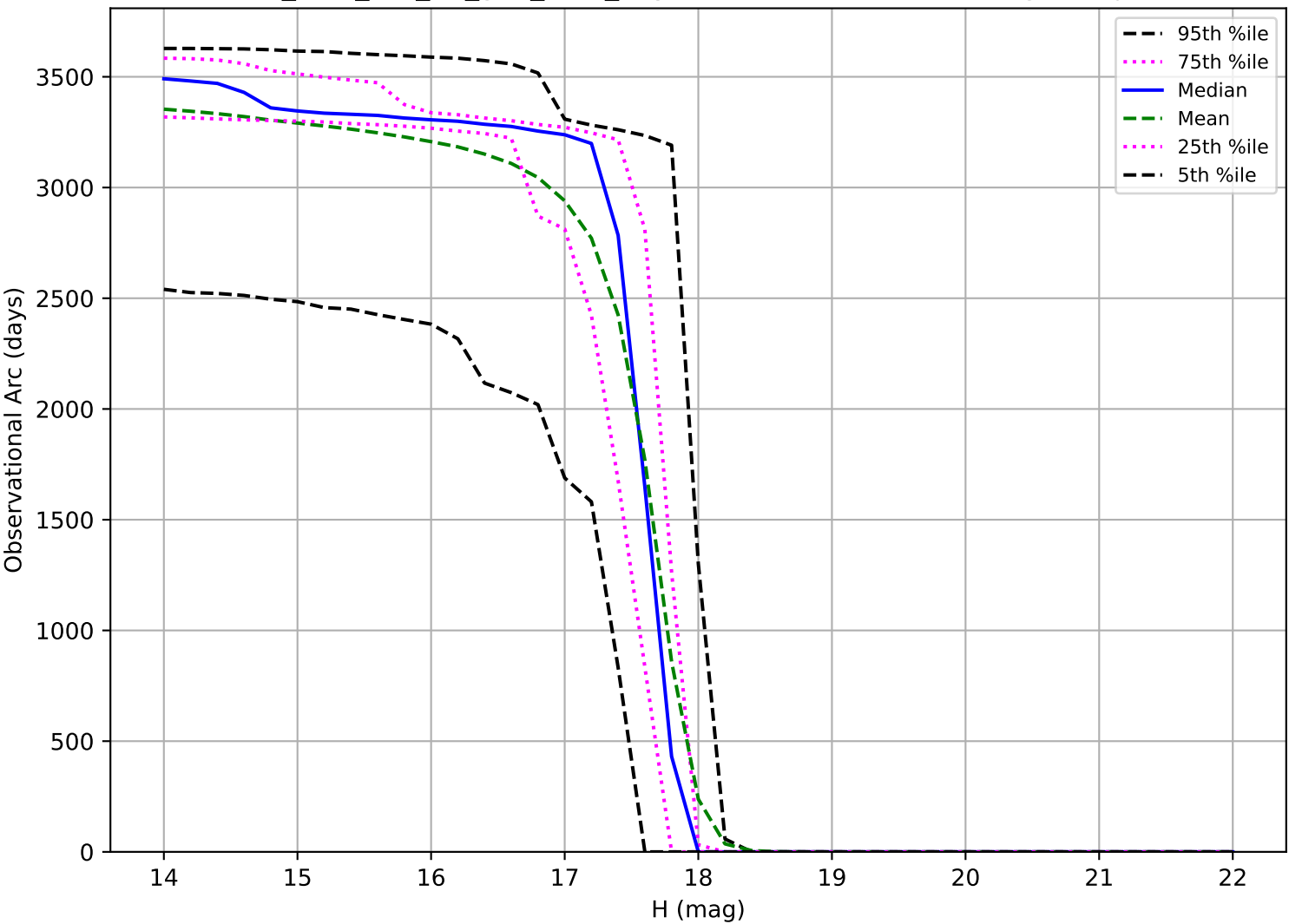
too_elab_r32_d3_griz_v3.4_10yrs: Observational Arc Length Trojan
