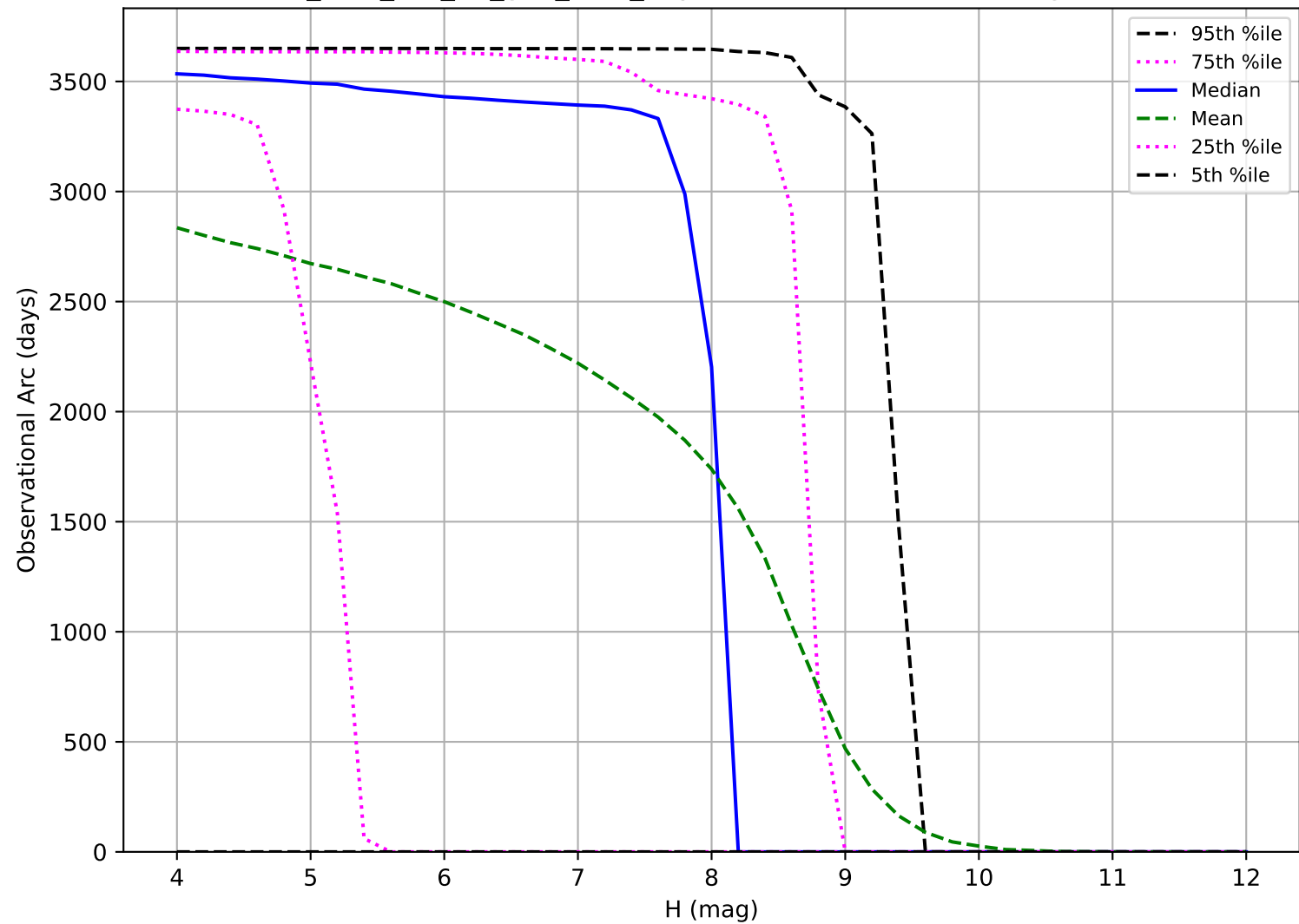
too_elab_r32_d3_griz_v3.4_10yrs: Observational Arc Length TNO
