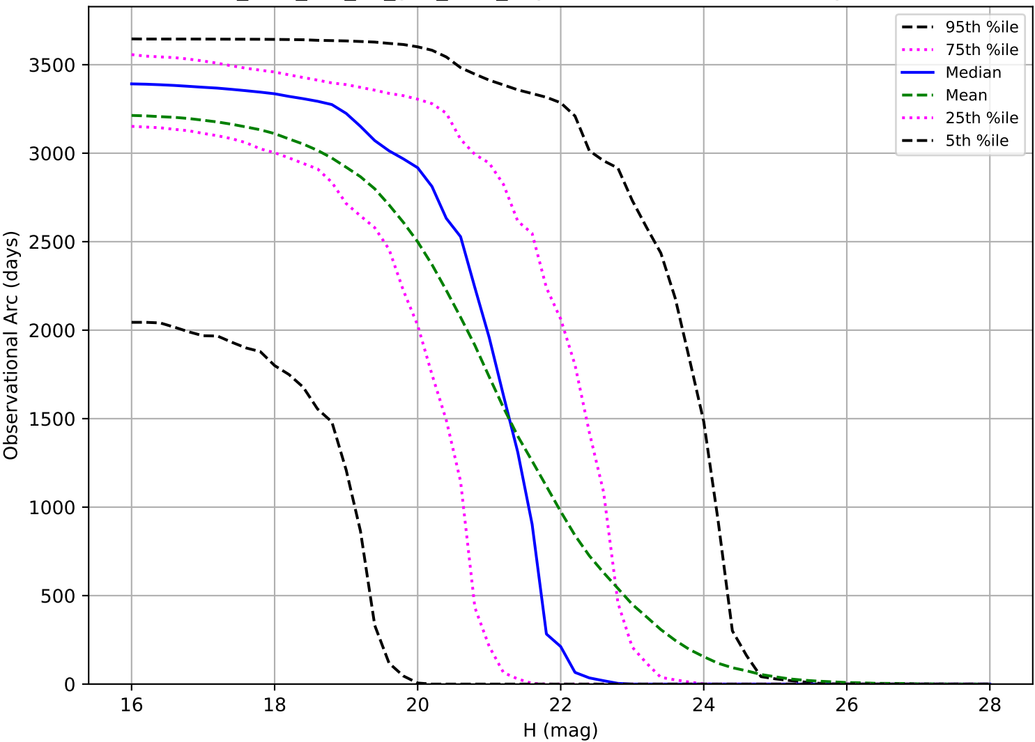
too_elab_r32_d3_griz_v3.4_10yrs: Observational Arc Length PHA
