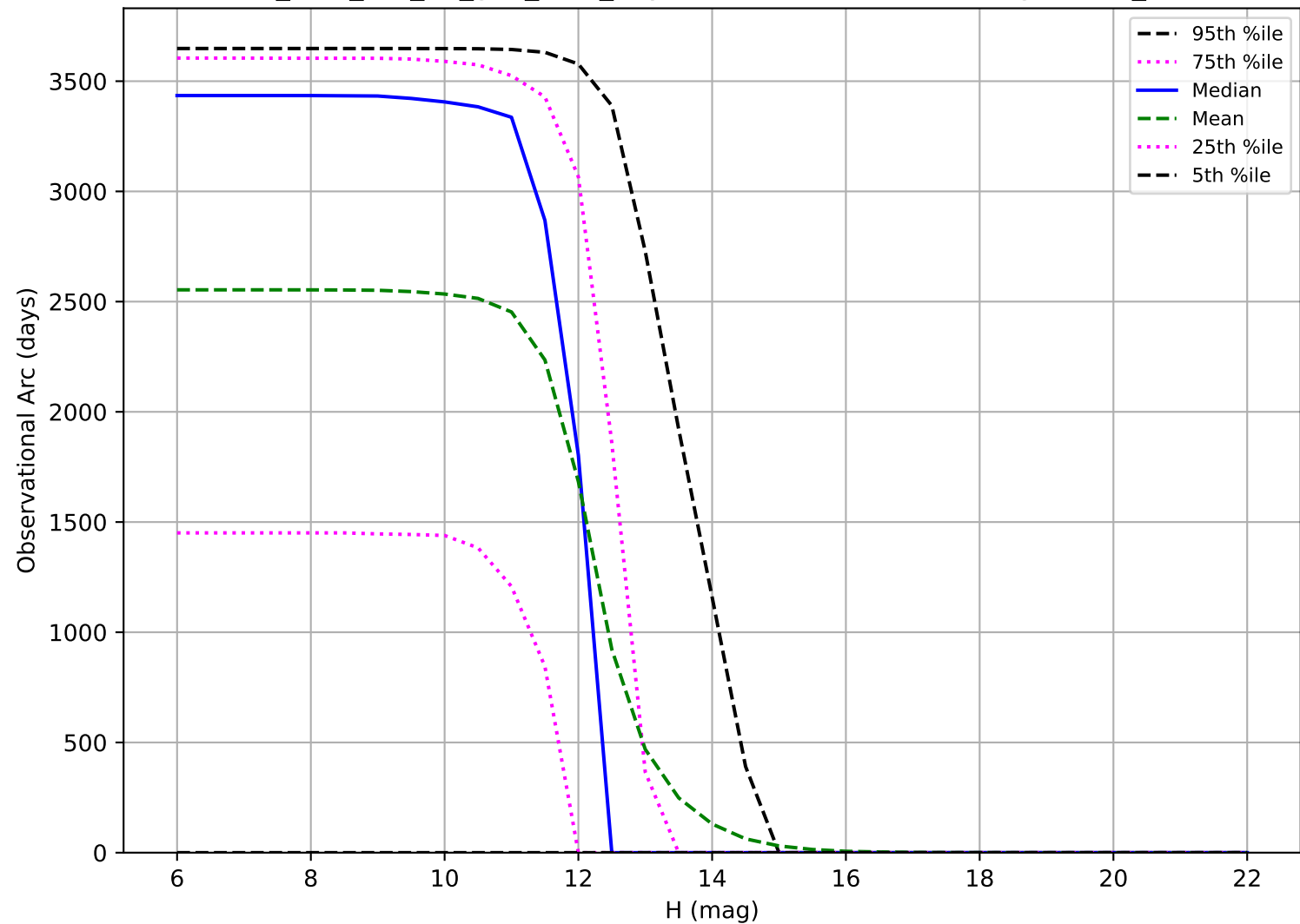
too_elab_r32_d3_griz_v3.4_10yrs: Observational Arc Length OCC_r20
