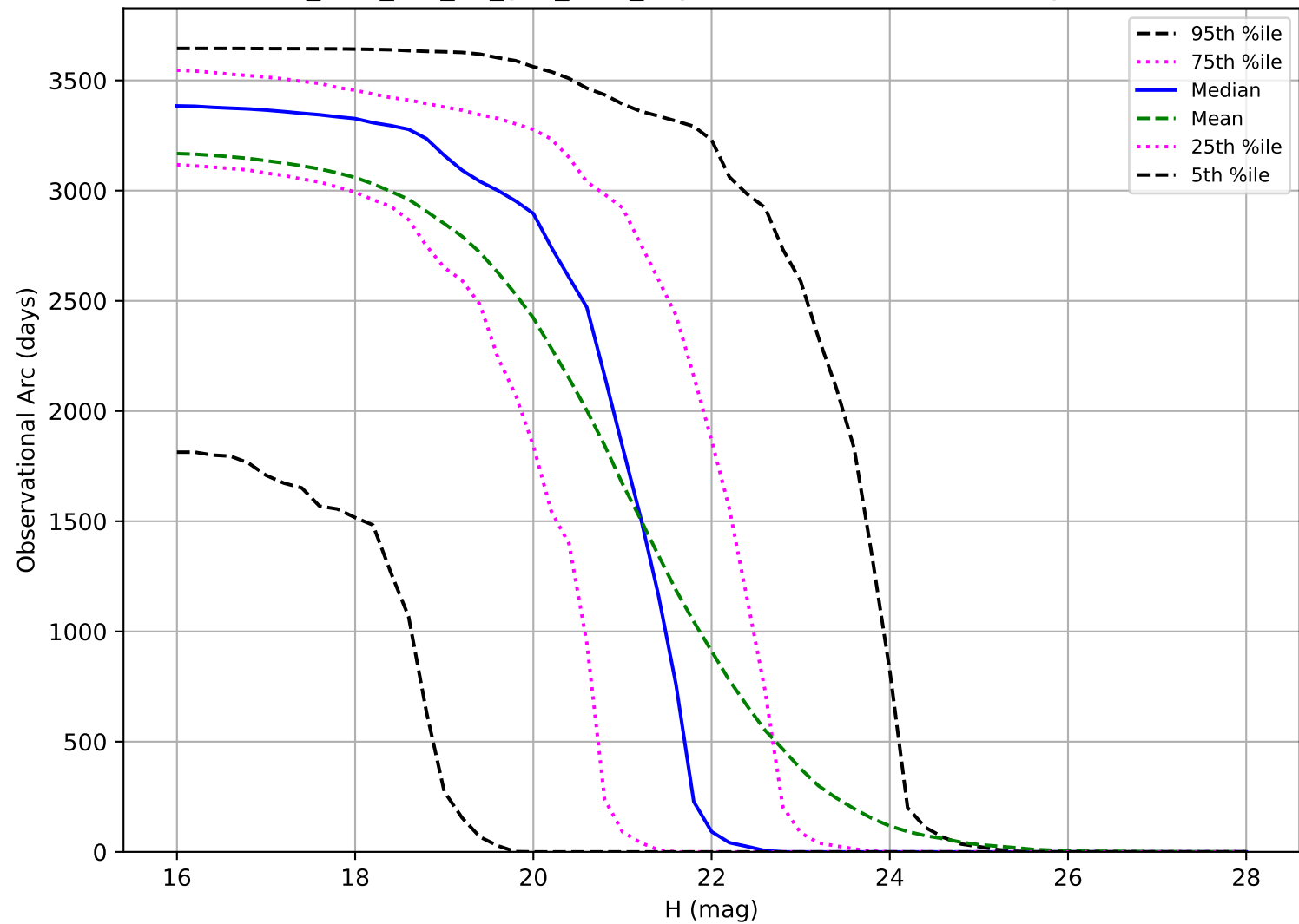
too_elab_r32_d3_griz_v3.4_10yrs: Observational Arc Length NEO
