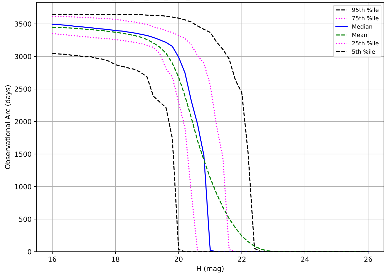
too_elab_r32_d3_griz_v3.4_10yrs: Observational Arc Length MBA
