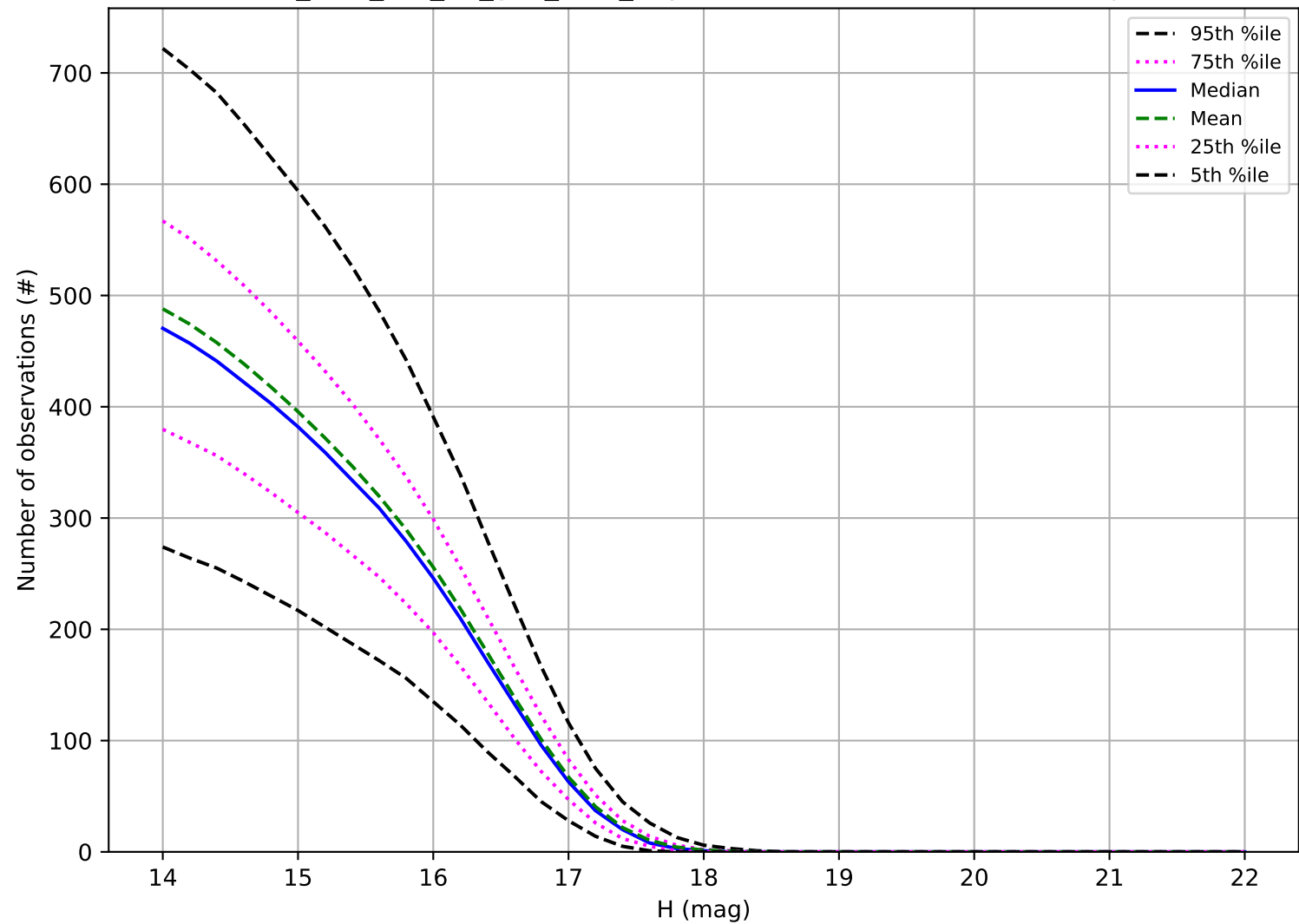
too_elab_r32_d3_griz_v3.4_10yrs: Number of observations Trojan
