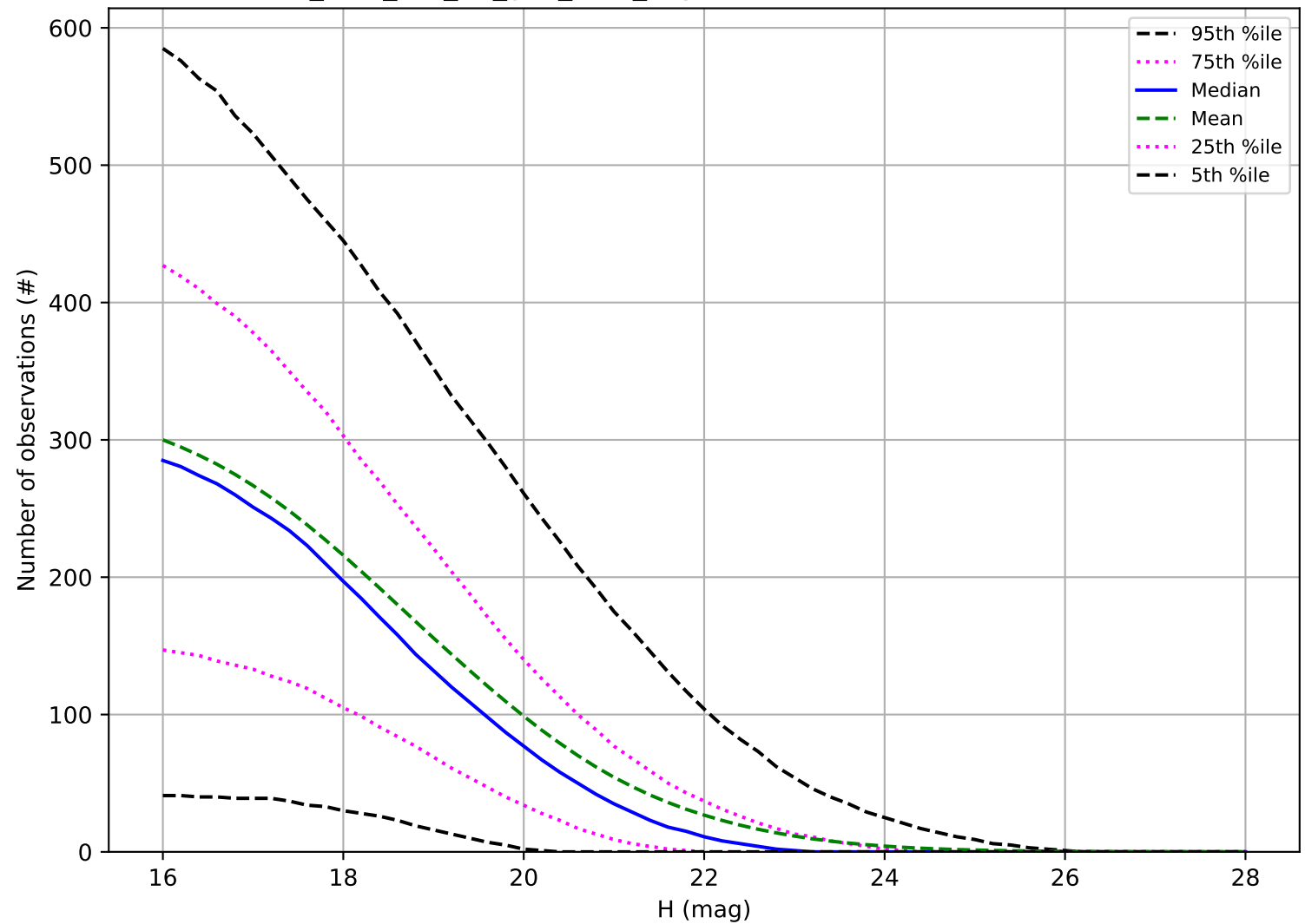
too_elab_r32_d3_griz_v3.4_10yrs: Number of observations PHA
