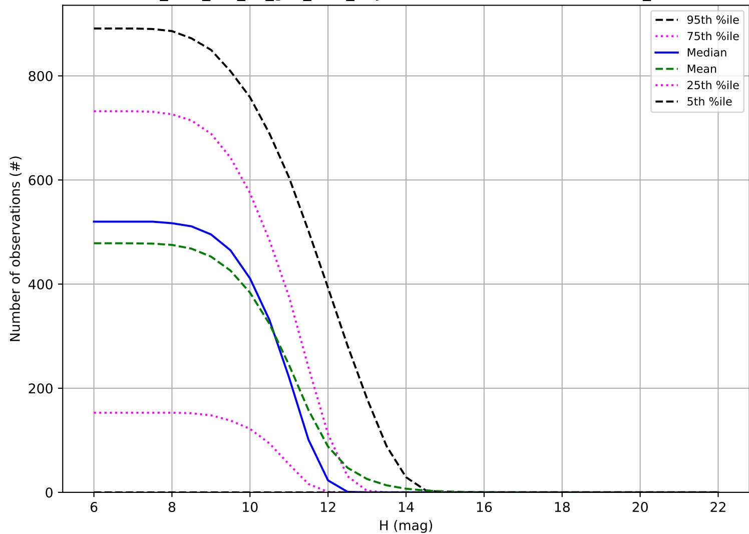
too_elab_r32_d3_griz_v3.4_10yrs: Number of observations OCC_r20
