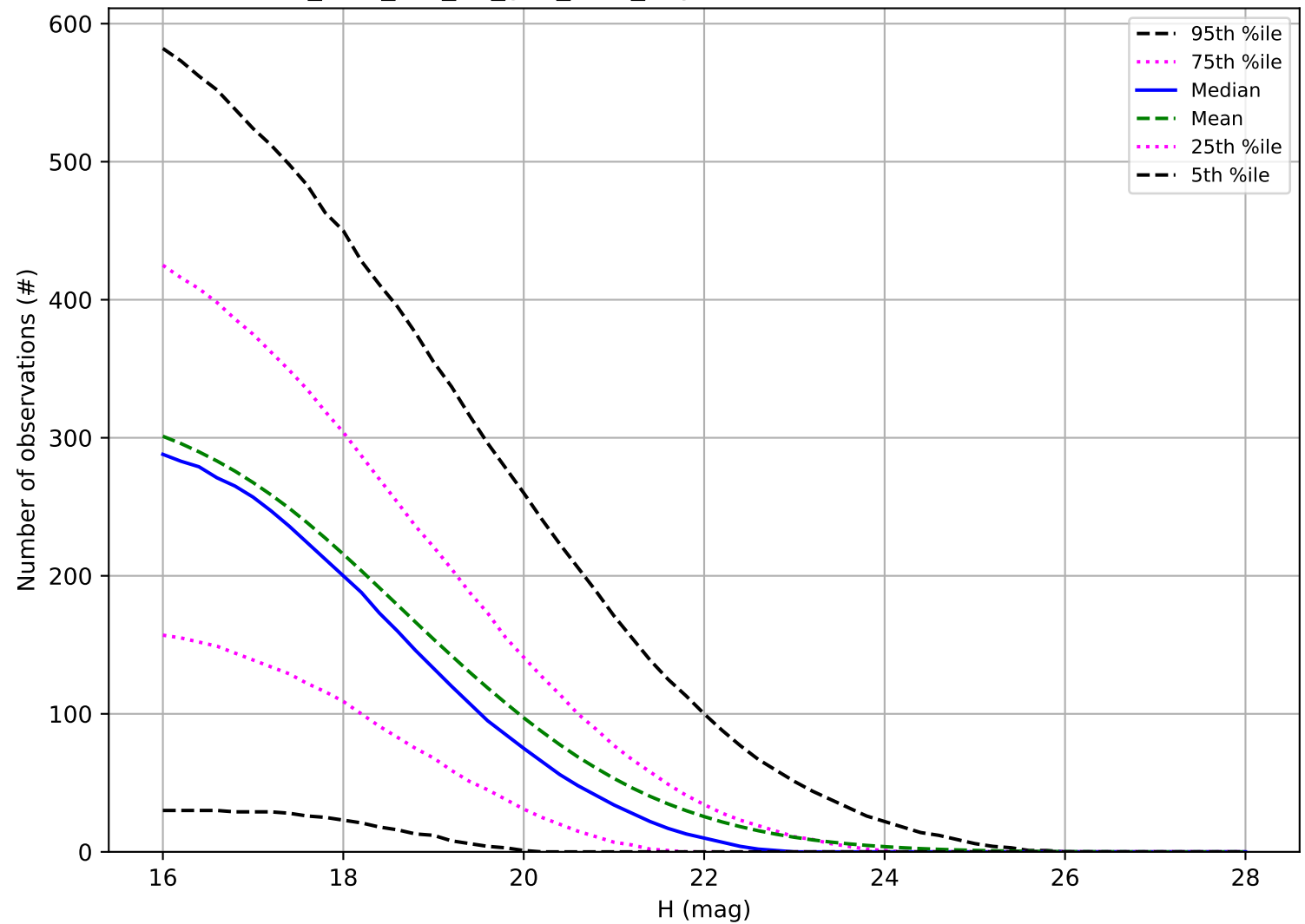
too_elab_r32_d3_griz_v3.4_10yrs: Number of observations NEO
