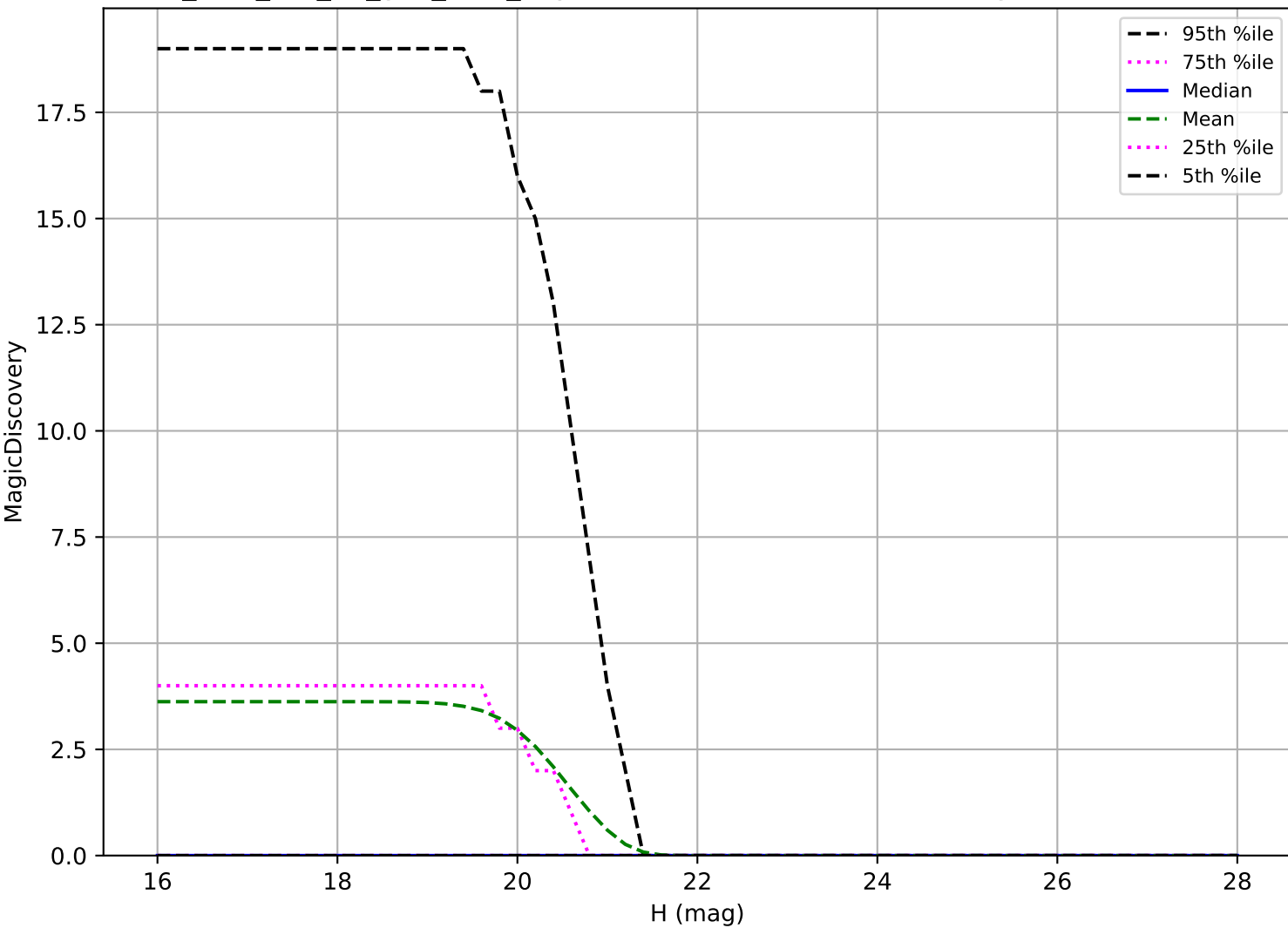
too_elab_r32_d3_griz_v3.4_10yrs: Vatira 6 detections in 60 nights detection loss
