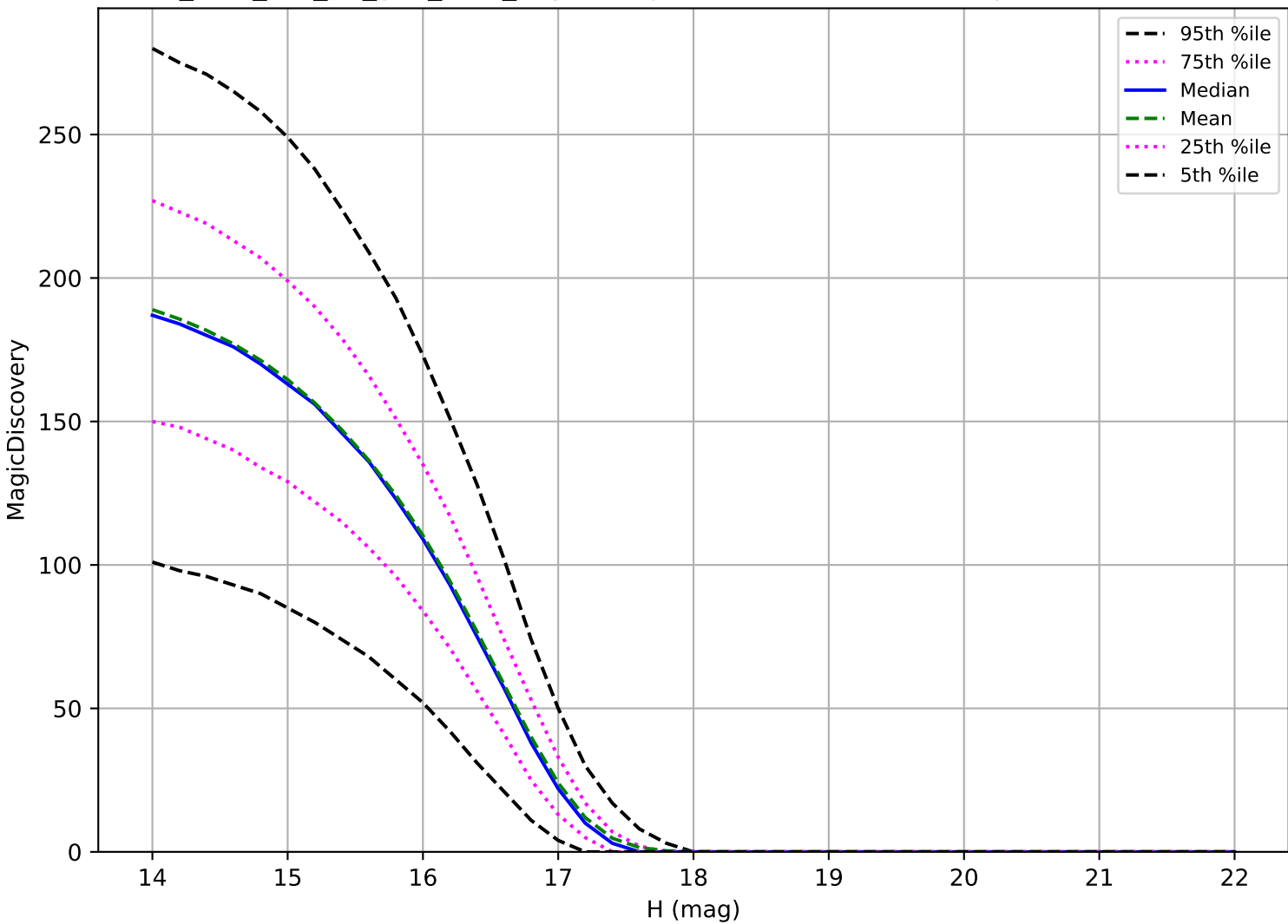
too_elab_r32_d3_griz_v3.4_10yrs: Trojan 6 detections in 60 nights detection loss
