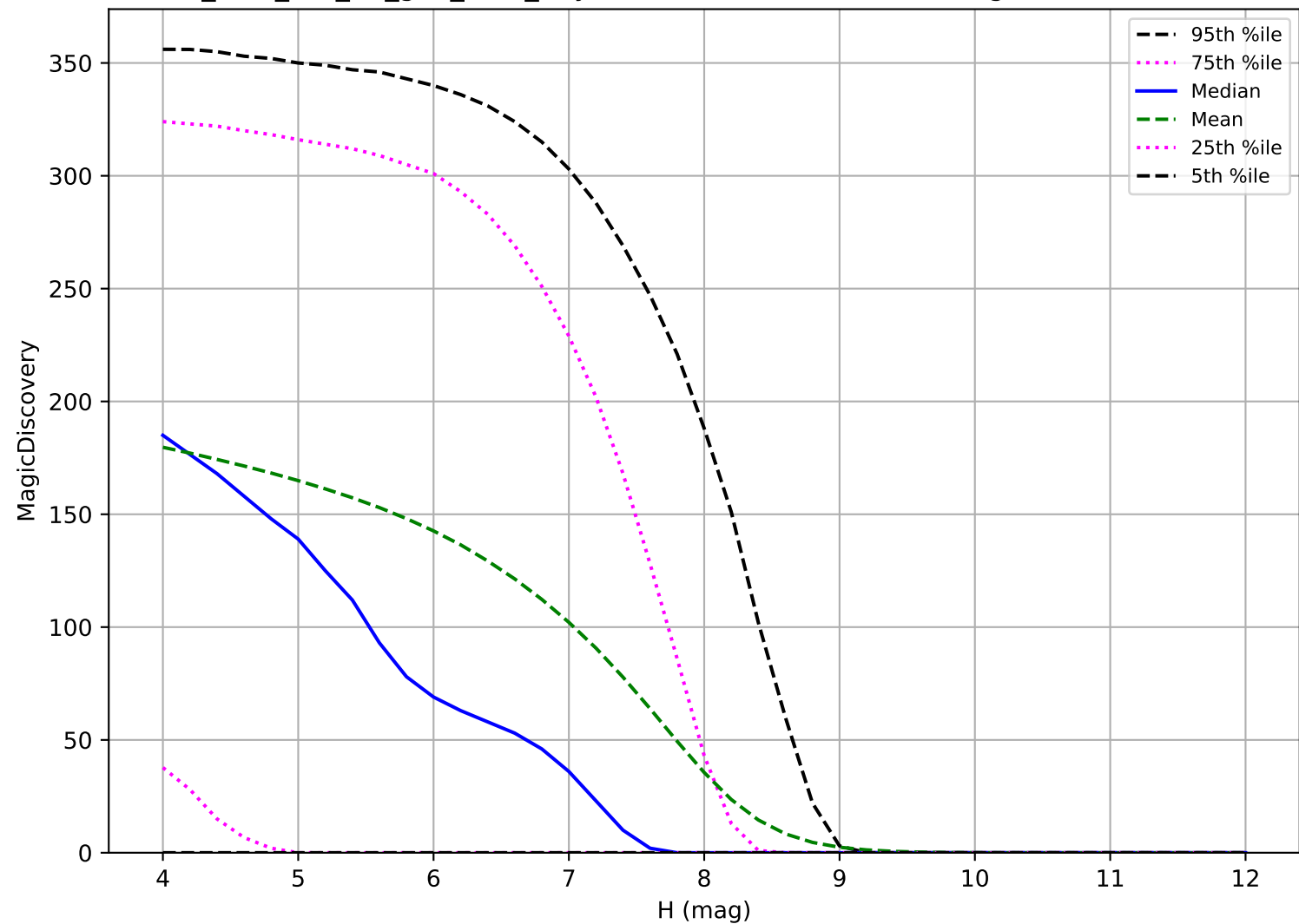
too_elab_r32_d3_griz_v3.4_10yrs: TNO 6 detections in 60 nights detection loss
