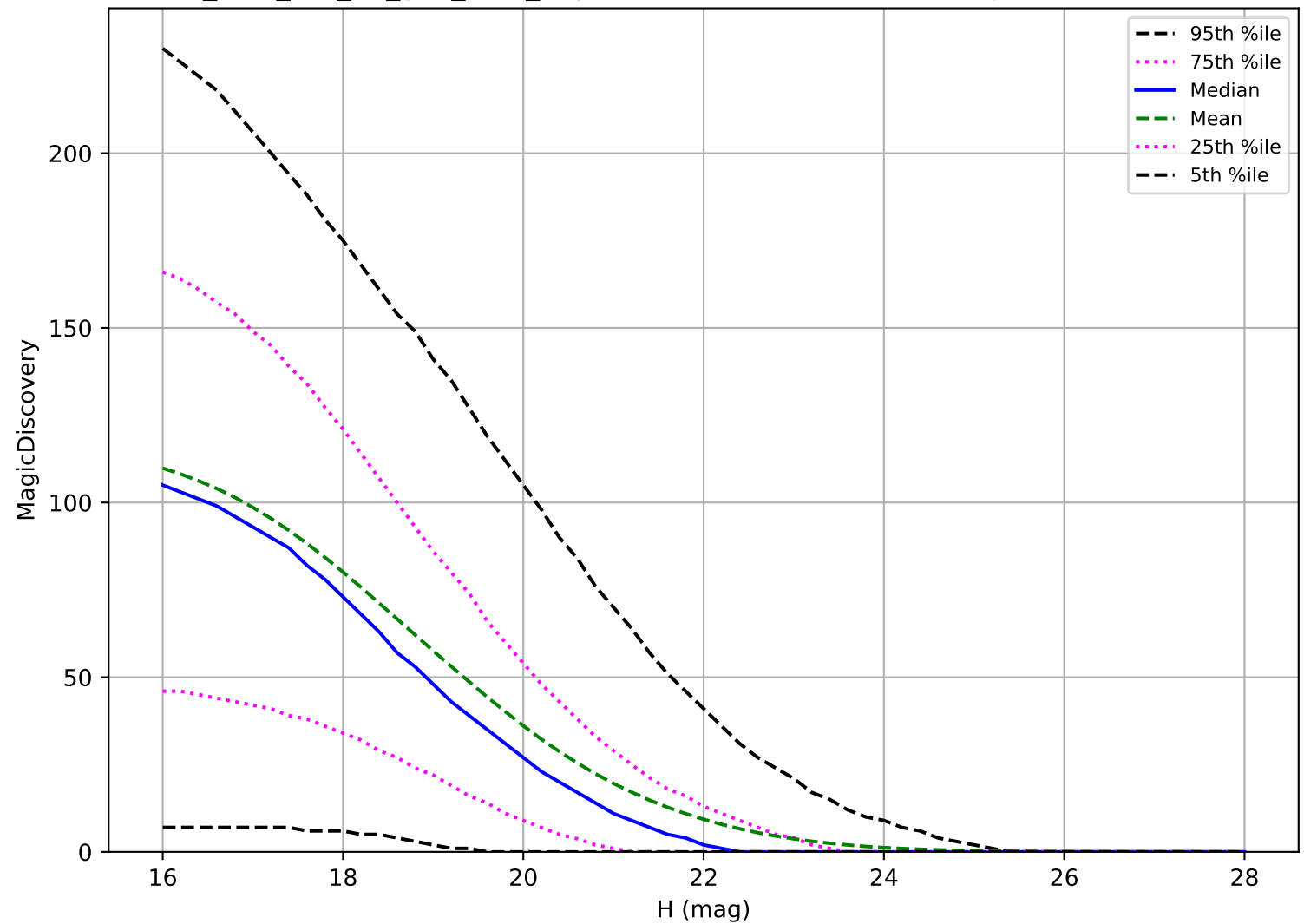
too_elab_r32_d3_griz_v3.4_10yrs: PHA 6 detections in 60 nights detection loss
