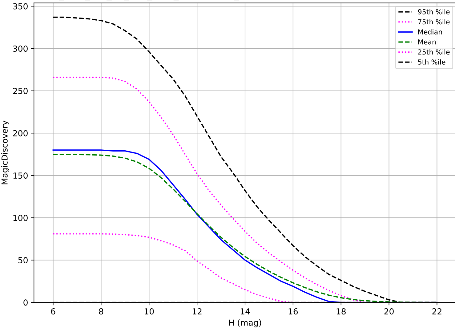
too_elab_r32_d3_griz_v3.4_10yrs: OCC_r5 6 detections in 60 nights detection loss
