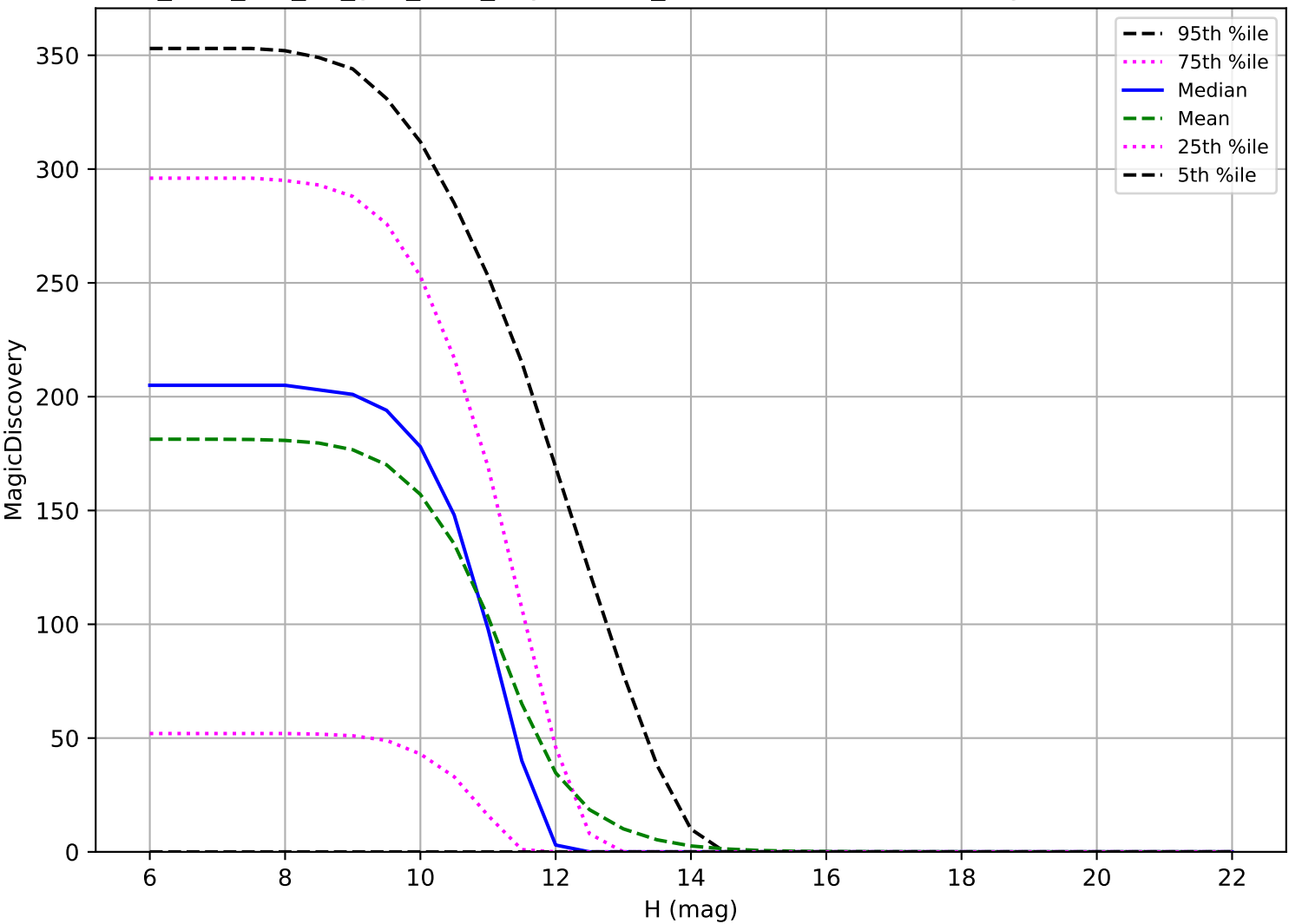
too_elab_r32_d3_griz_v3.4_10yrs: OCC_r20 6 detections in 60 nights detection loss
