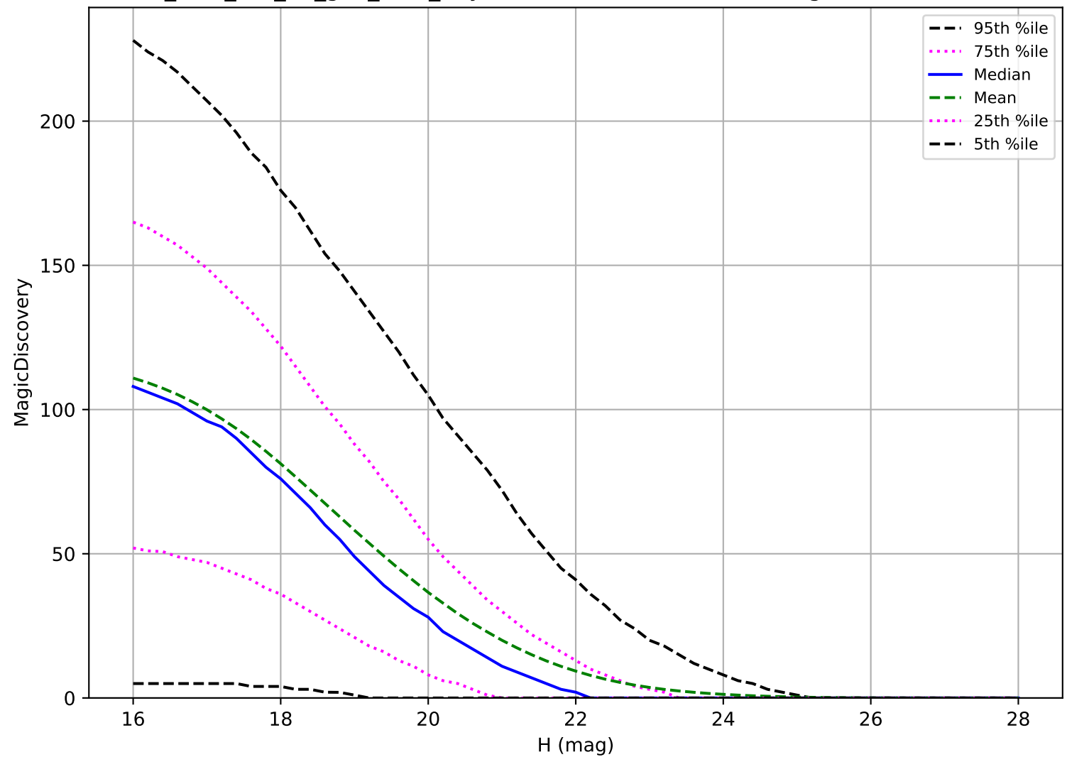
too_elab_r32_d3_griz_v3.4_10yrs: NEO 6 detections in 60 nights detection loss
