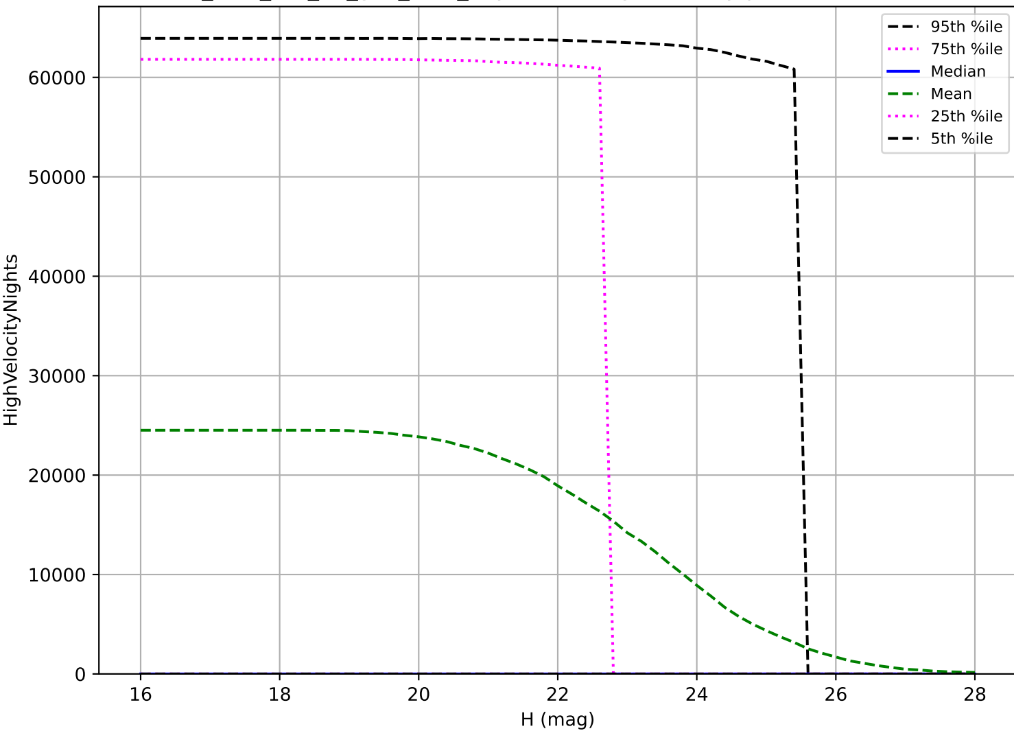
too_elab_r32_d3_griz_v3.4_10yrs: PHA High velocity pair detection loss
