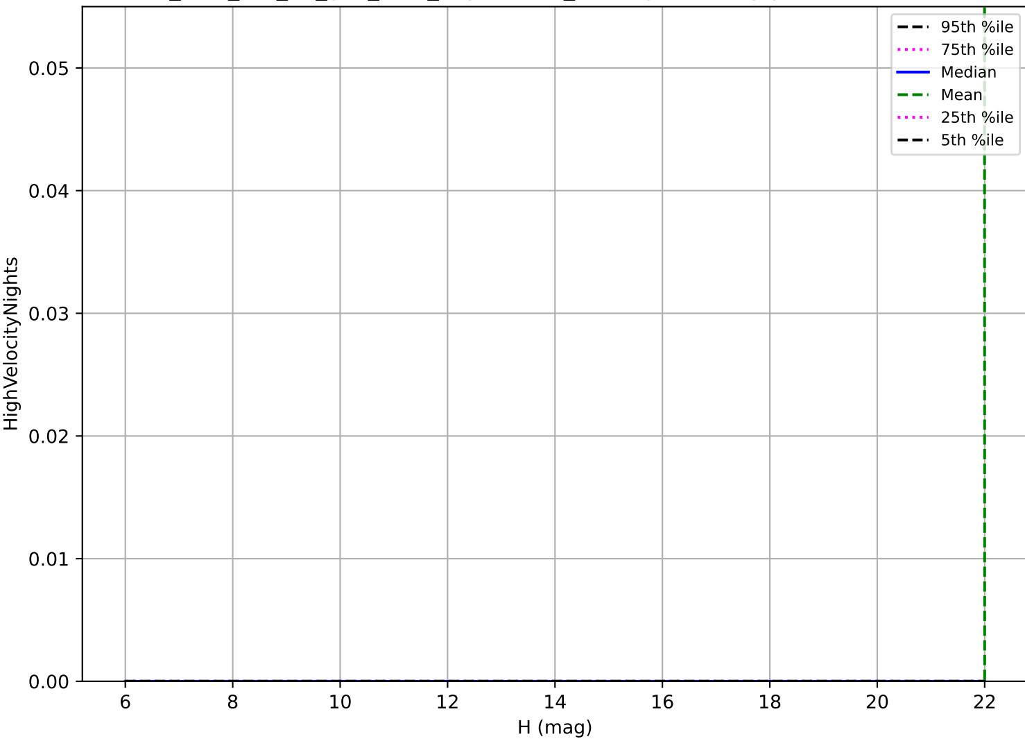
too_elab_r32_d3_griz_v3.4_10yrs: OCC_r20 High velocity pair detection loss
