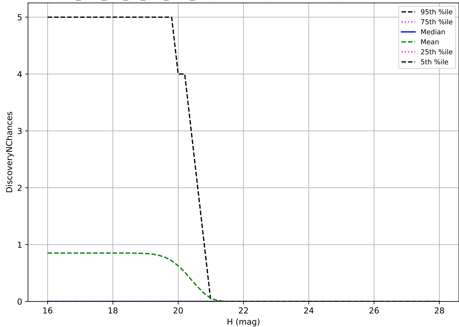
too_elab_r32_d3_griz_v3.4_10yrs: Vatira 3 pairs in 15 nights detection loss
