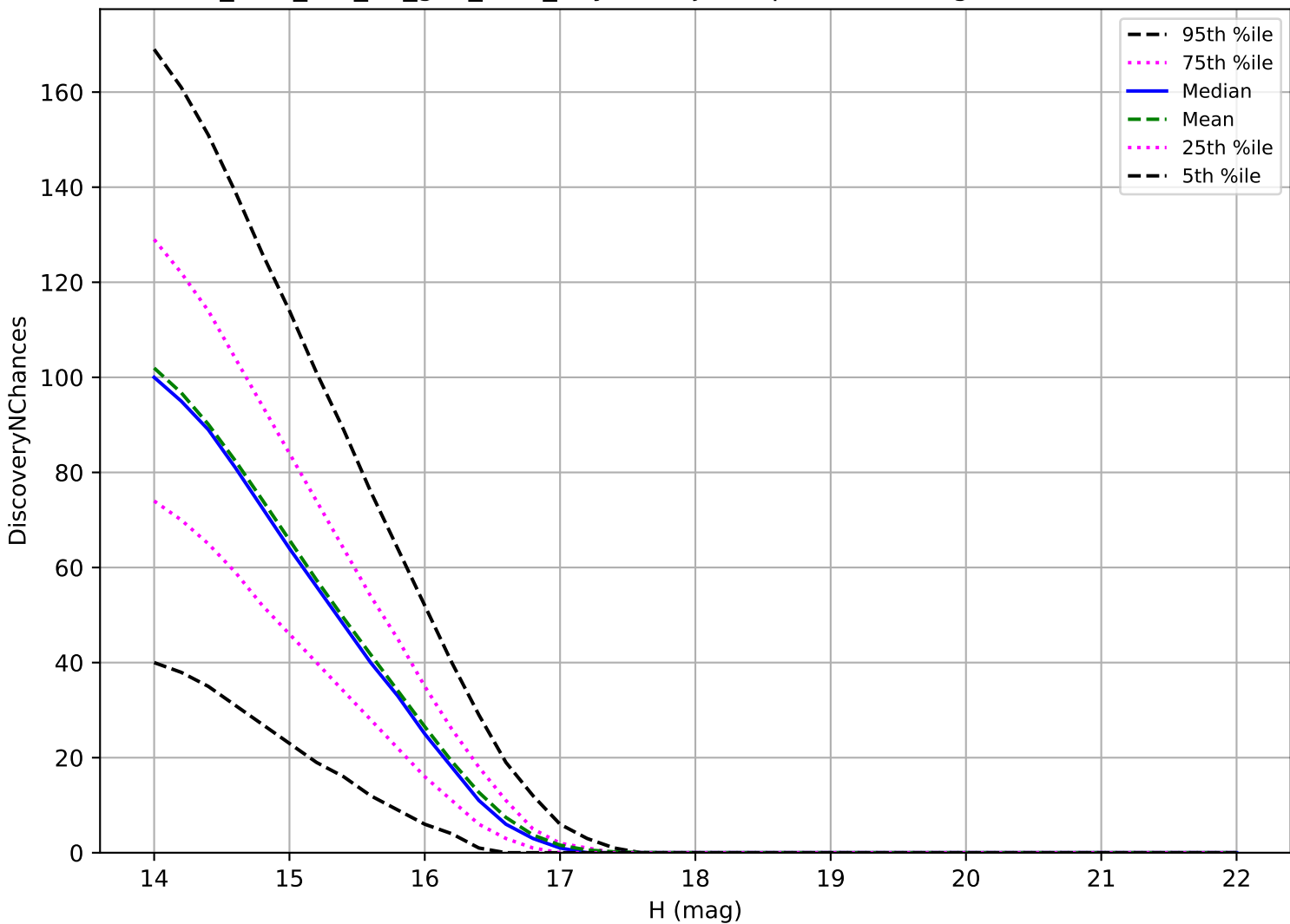
too_elab_r32_d3_griz_v3.4_10yrs: Trojan 3 pairs in 15 nights detection loss
