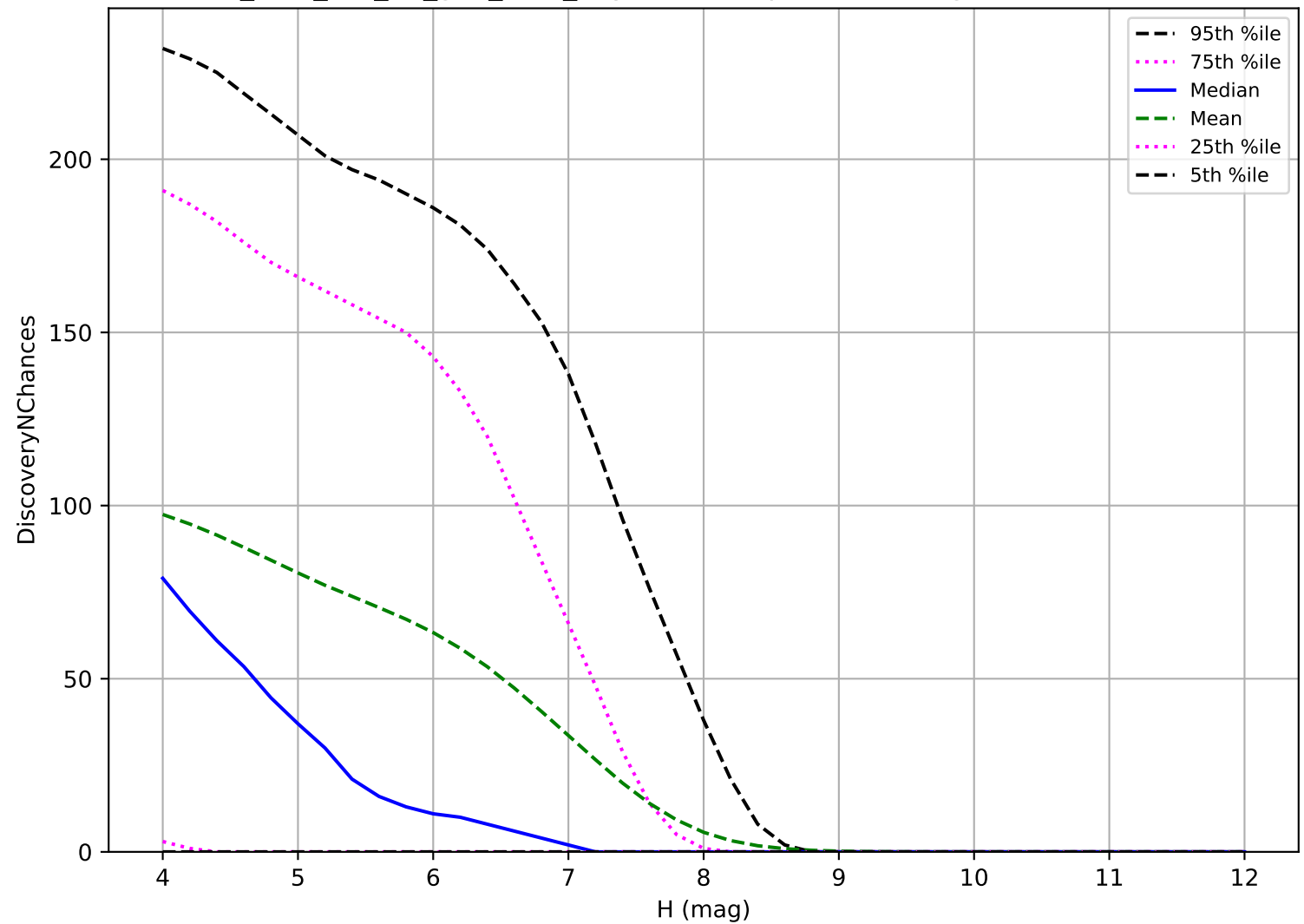
too_elab_r32_d3_griz_v3.4_10yrs: TNO 3 pairs in 15 nights detection loss
