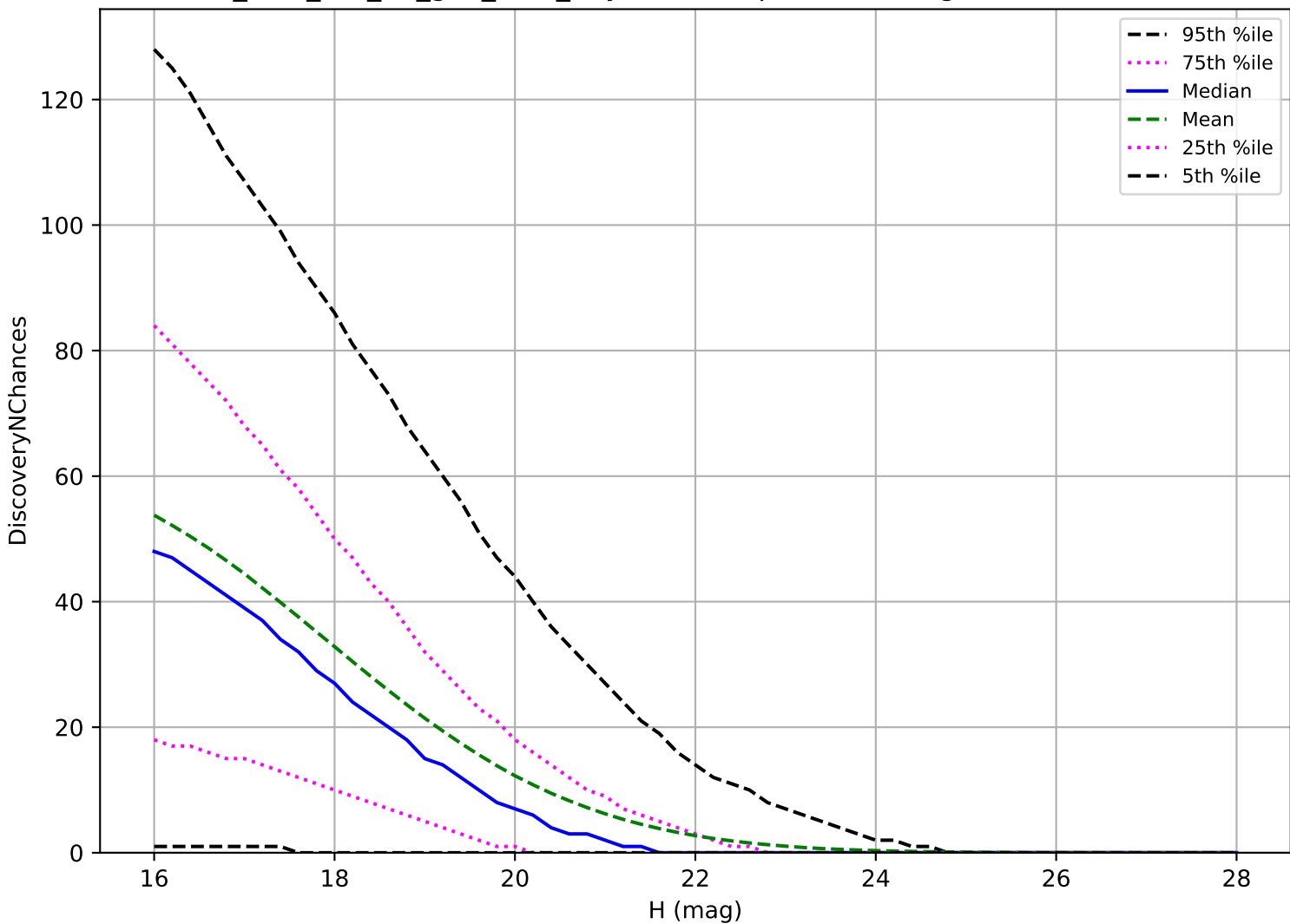
too_elab_r32_d3_griz_v3.4_10yrs: PHA 3 pairs in 15 nights detection loss
