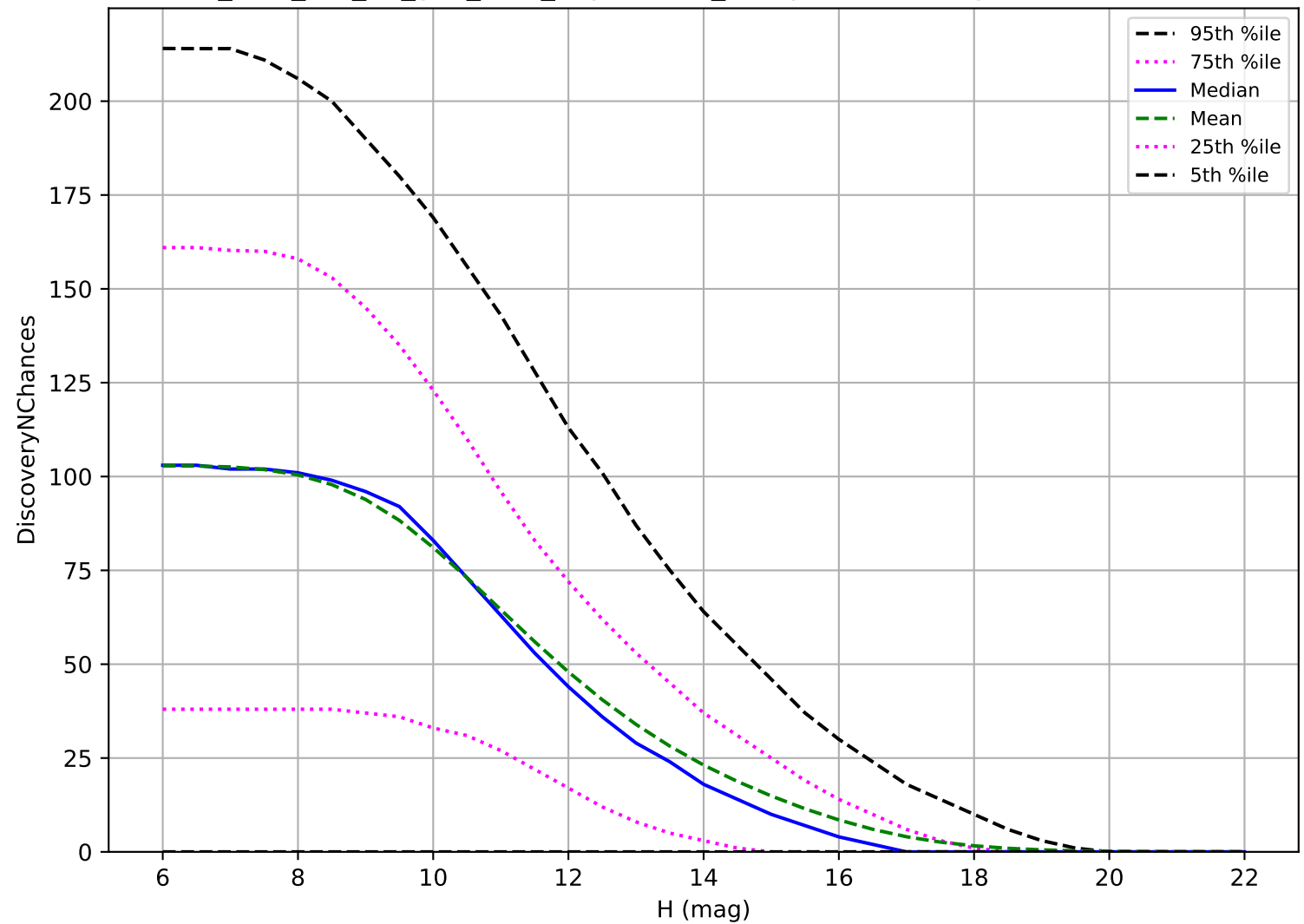
too_elab_r32_d3_griz_v3.4_10yrs: OCC_r5 3 pairs in 15 nights detection loss
