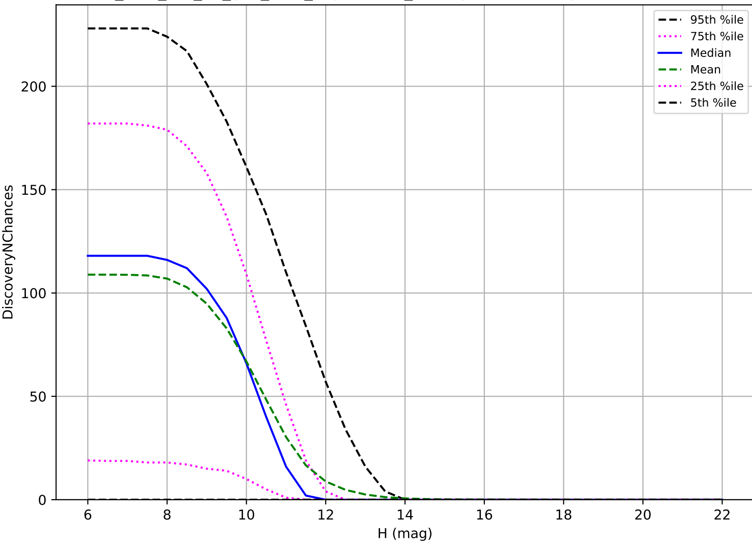
too_elab_r32_d3_griz_v3.4_10yrs: OCC_r20 3 pairs in 15 nights detection loss
