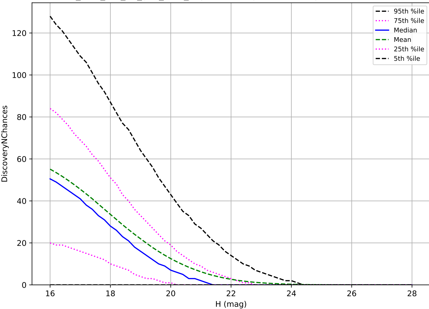
too_elab_r32_d3_griz_v3.4_10yrs: NEO 3 pairs in 15 nights detection loss
