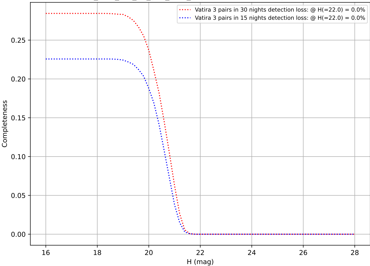
too_elab_r32_d3_griz_v3.4_10yrs: DifferentialCompleteness
