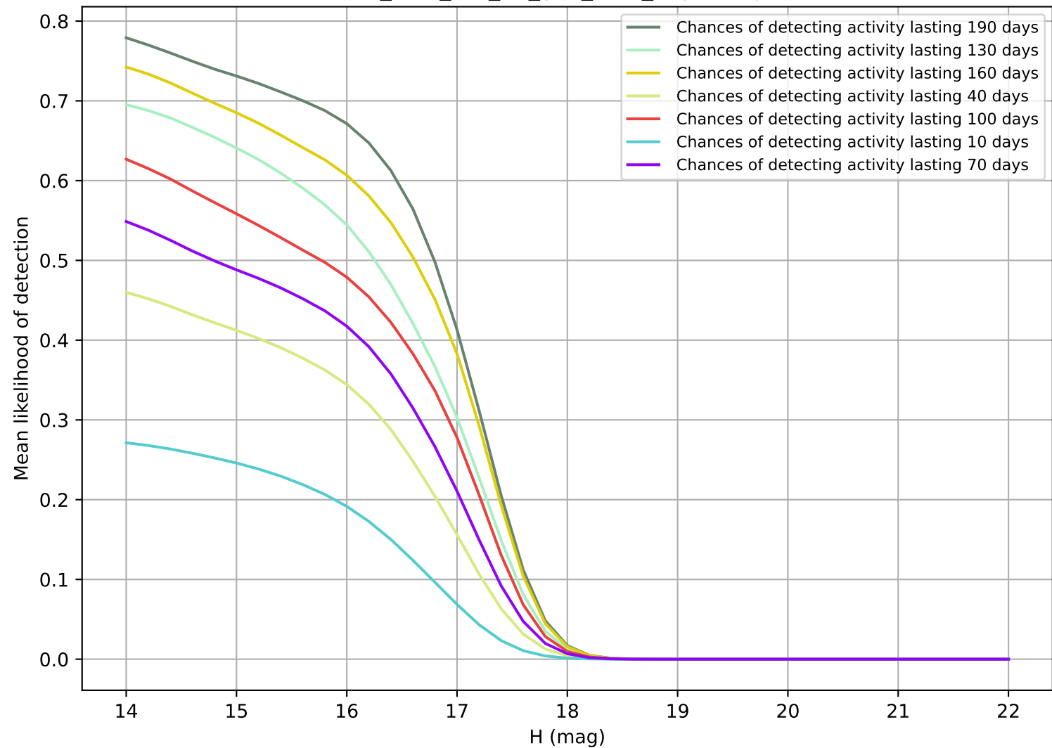
too_elab_r32_d3_griz_v3.4_10yrs Trojan
