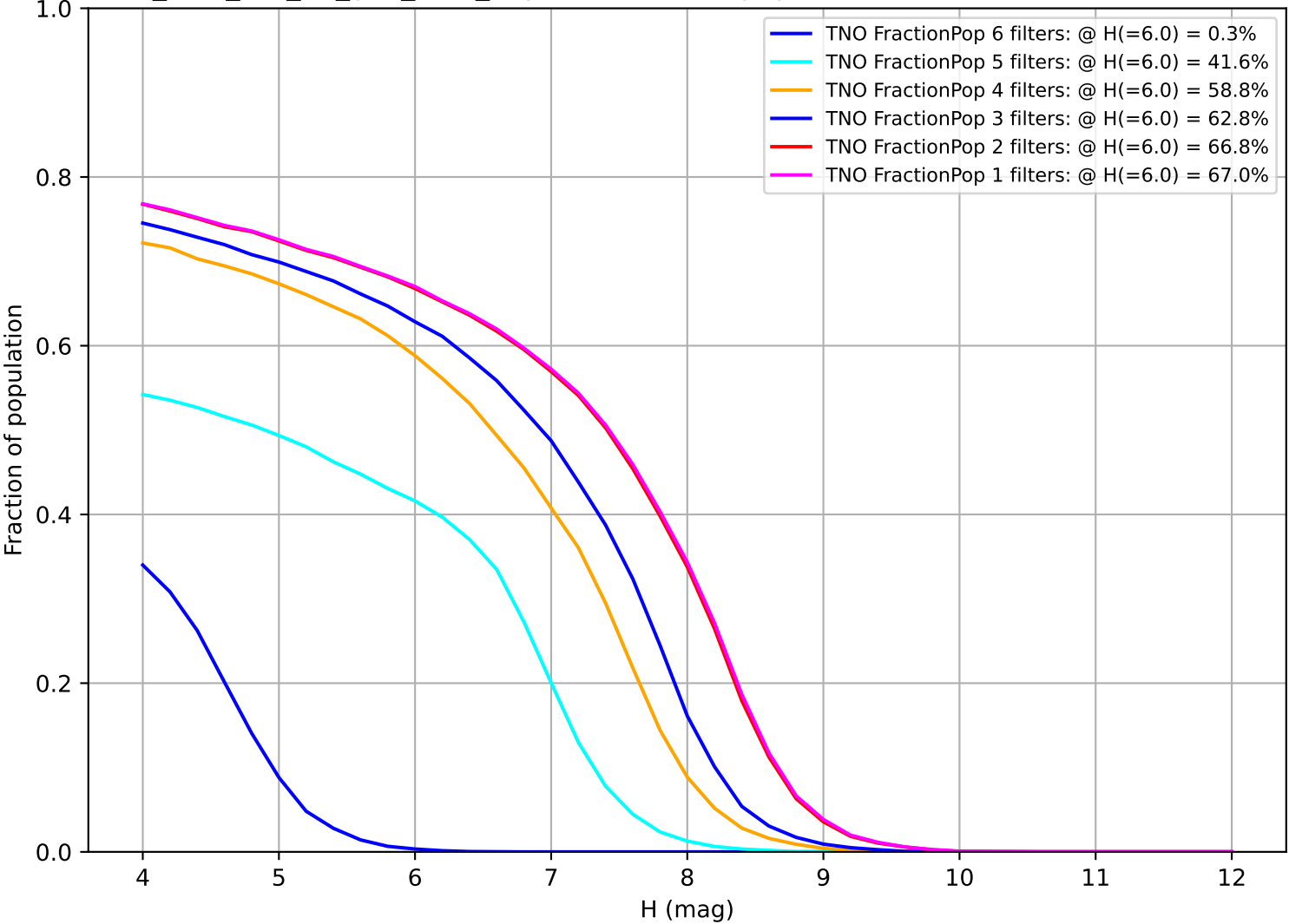
too_elab_r32_d3_griz_v3.4_10yrs: Fraction of population with colors in X filters TNO
