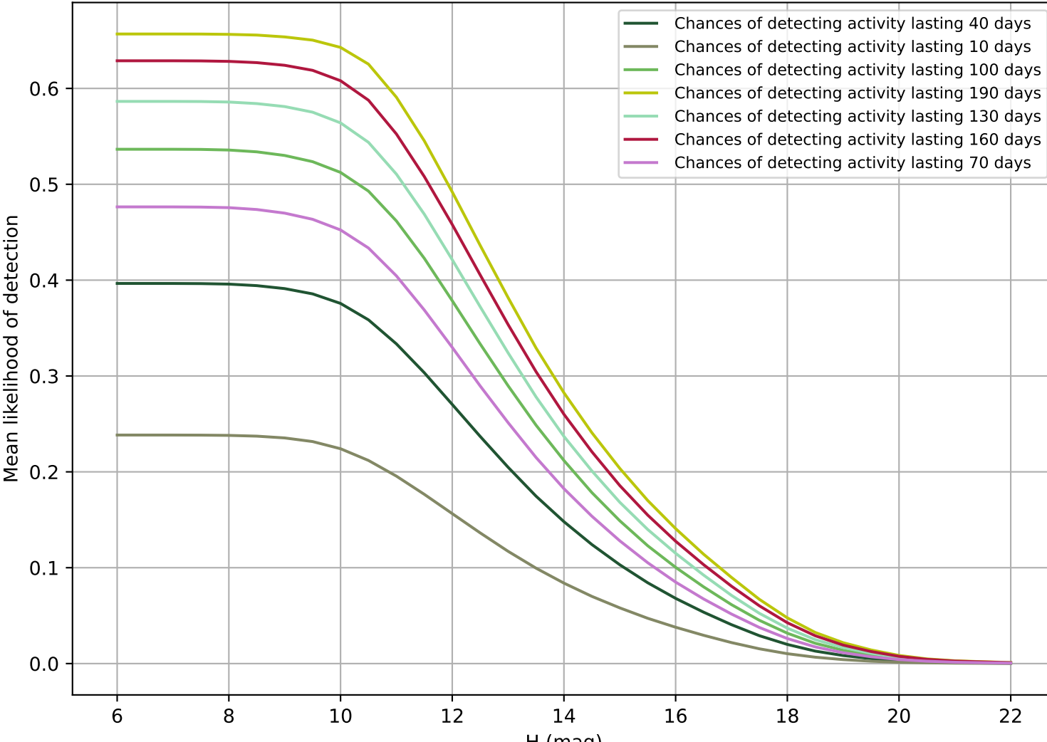
too_elab_r32_d3_griz_v3.4_10yrs OCC_r5
