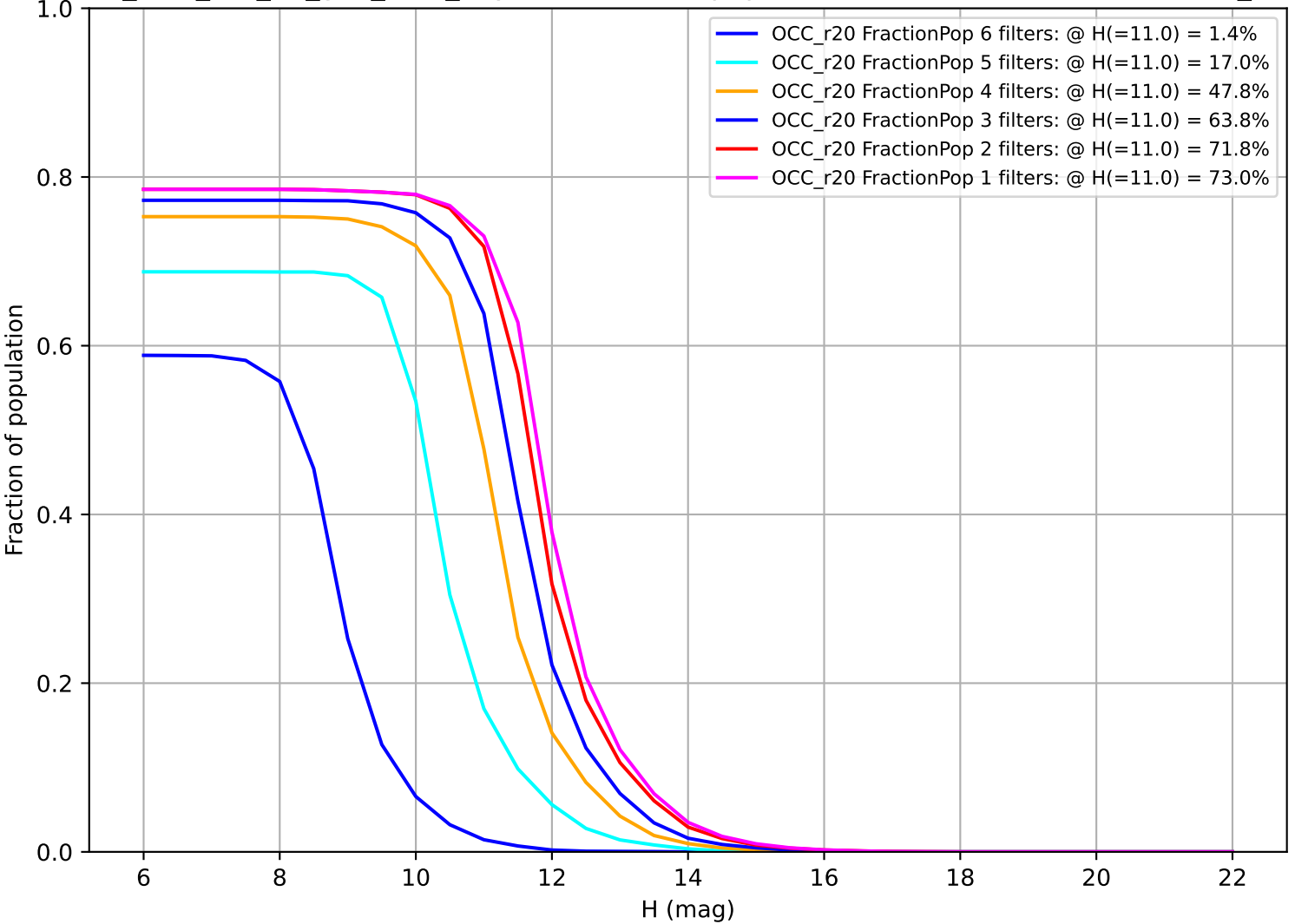
too_elab_r32_d3_griz_v3.4_10yrs: Fraction of population with colors in X filters OCC_r20
