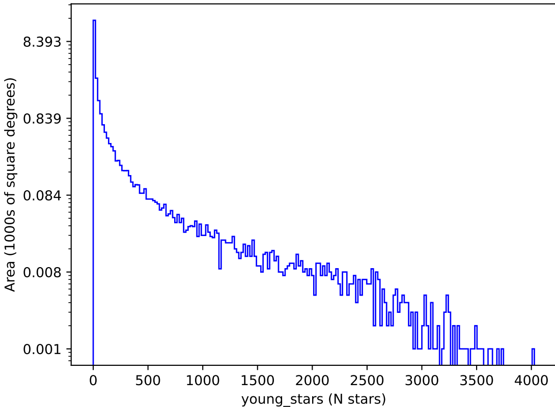
too_elab_r32_d3_griz_v3.4_10yrs : young_stars
