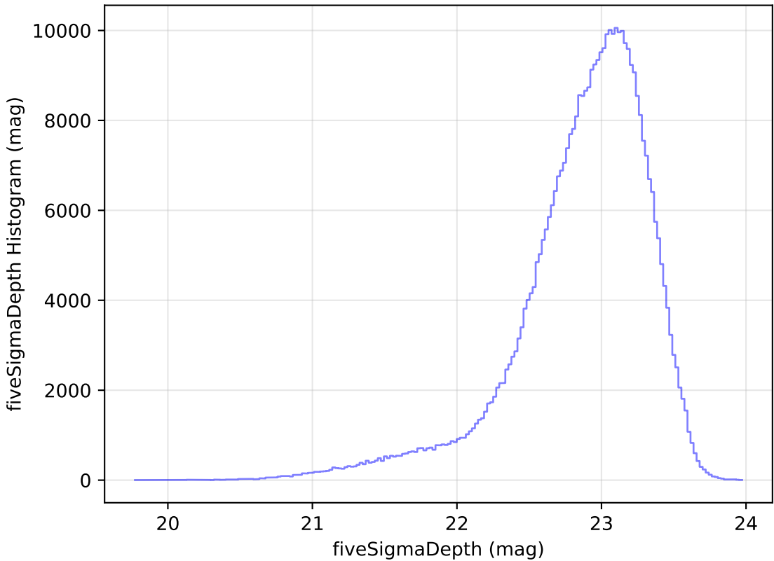
too_elab_r32_d3_griz_v3.4_10yrs z: fiveSigmaDepth Histogram
