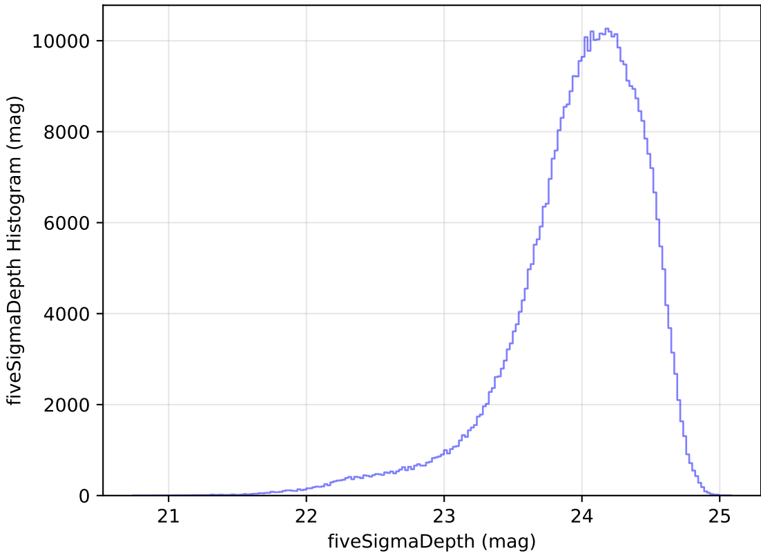
too_elab_r32_d3_griz_v3.4_10yrs r: fiveSigmaDepth Histogram
