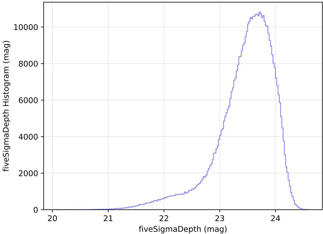
too_elab_r32_d3_griz_v3.4_10yrs i: fiveSigmaDepth Histogram
