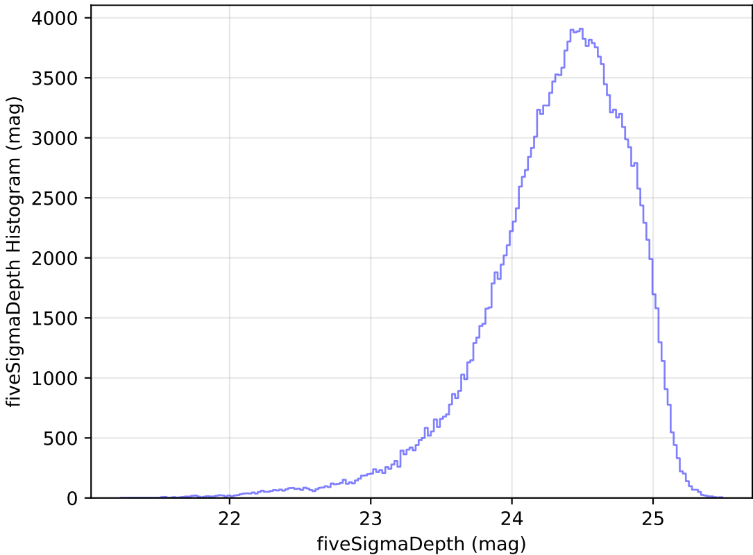
too_elab_r32_d3_griz_v3.4_10yrs g: fiveSigmaDepth Histogram
