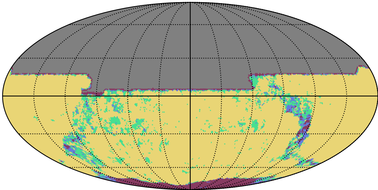
too_elab_r32_d3_griz_v3.4_10yrs y band: YearCoverage night
