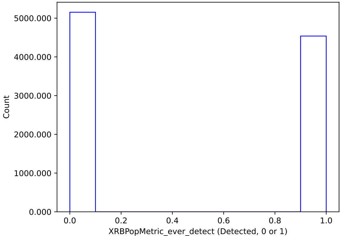
too_elab_r32_d3_griz_v3.4_10yrs : XRBPoMetric_ever_detect
