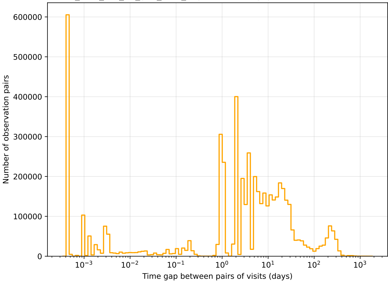
too_elab_r32_d3_griz_v3.4_10yrs r band: Tgaps observationStartMJD
